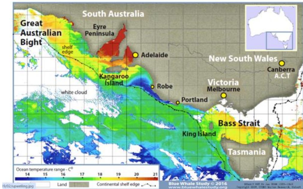
Figure.5. - Typical Surface Water Temperatures in Autumn (ref. Blue Whale Study)
