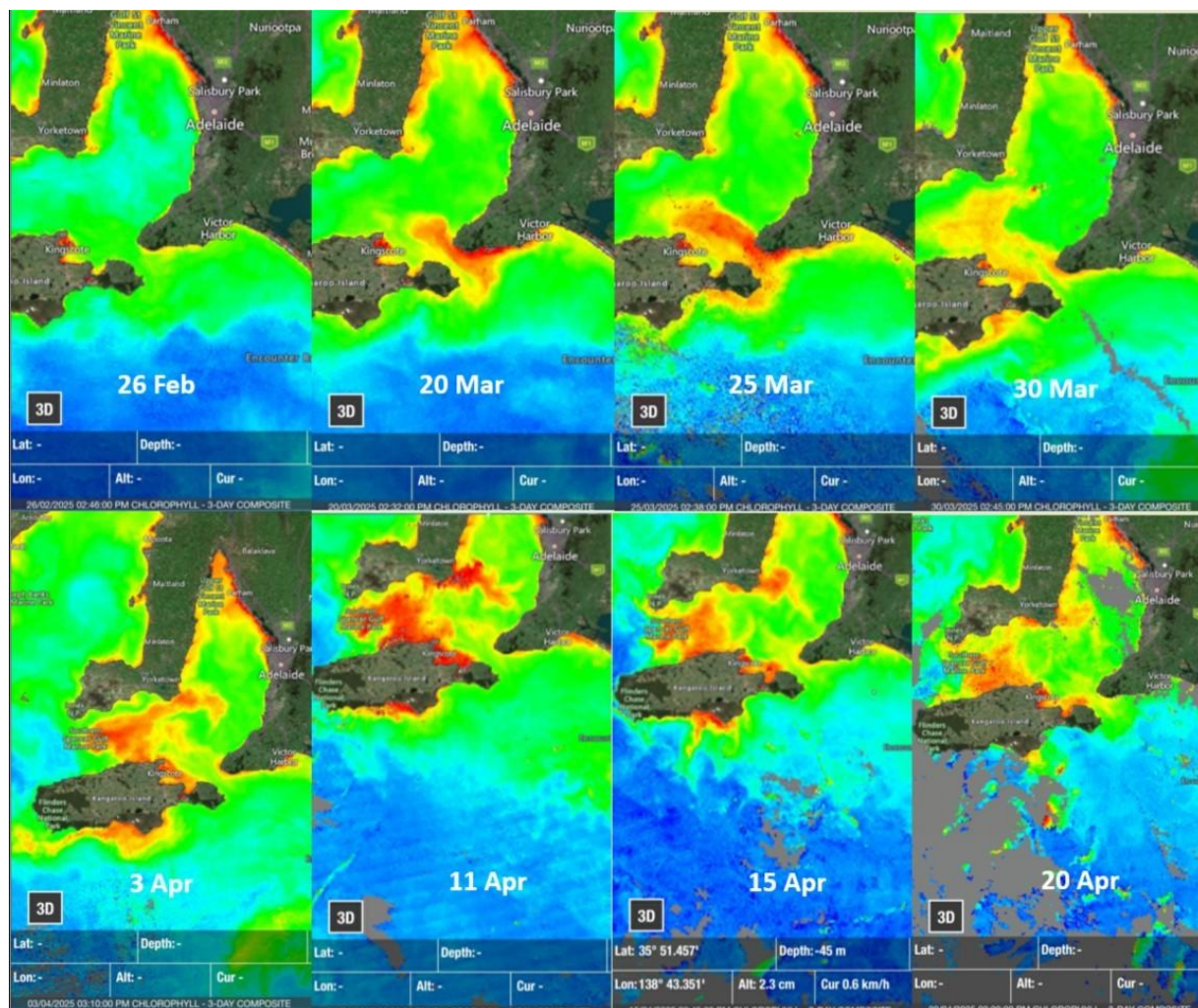
Fig.10. – HAB enters Gulf St Vincent (Chlor. A levels over Summer and Autumn 2025.)
