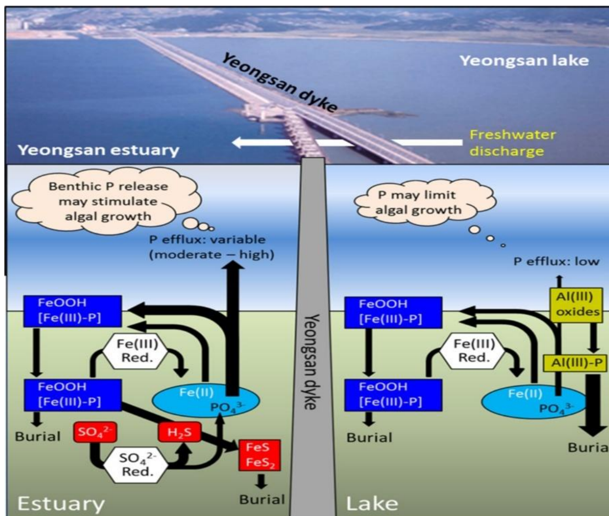
Figure. 7. – P Release from Sediment under Anoxic Conditions (An, et al, 2019)
