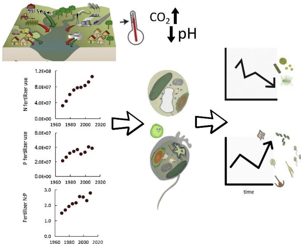
Figure.8. – Use of Fertilisers Favours Growth of Mixotrophs
